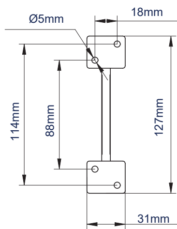
INTERFACE BRACKET
