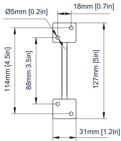
INTERFACE BRACKET
