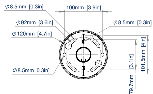
TOP VIEW CEILING MOUNTING PLATE
