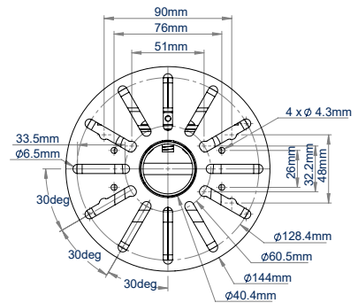
CAMERA MOUNT INTERFACE BOTTOM VIEW
