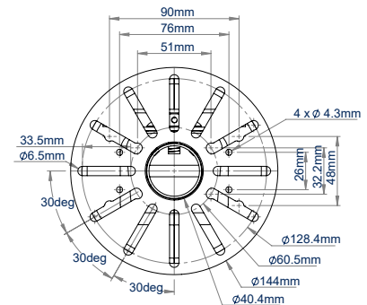
CAMERA MOUNT INTERFACE BOTTOM VIEW
