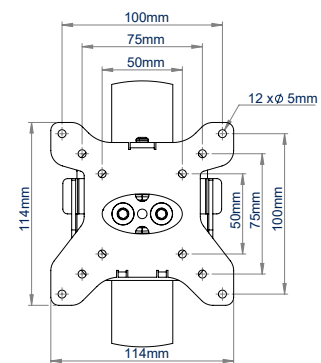
SCREEN MOUNT INTERFACE FRONT VIEW
