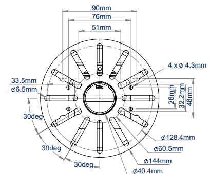
SCREEN MOUNT INTERFACE FRONT VIEW
