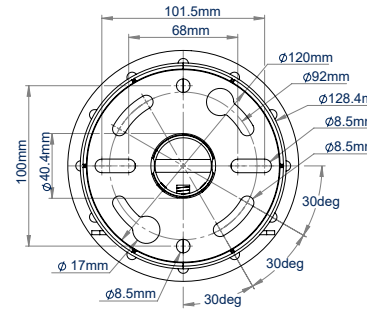
CEILING PLATE TOP VIEW
