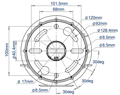
TOP VIEW CEILING PLATE
