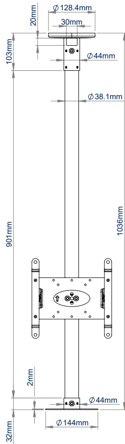
BT5964-FD100 FRONT VIEW
