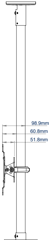
SIDE VIEW
