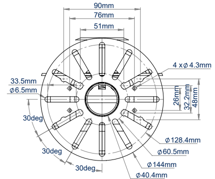
BOTTOM VIEW CCTV CAMERA MOUNT
