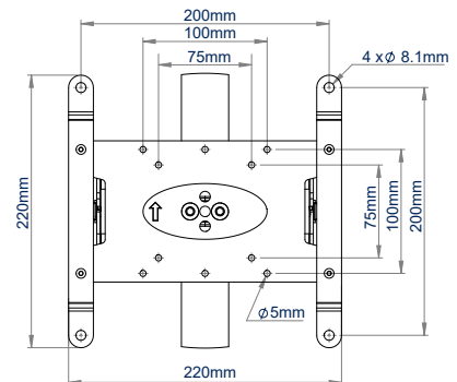
FRONT VIEW SCREEN MOUNT
