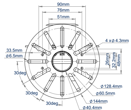
BOTTOM VIEW CCTV CAMERA MOUNT
