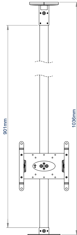
BT5964-FD200 FRONT VIEW
