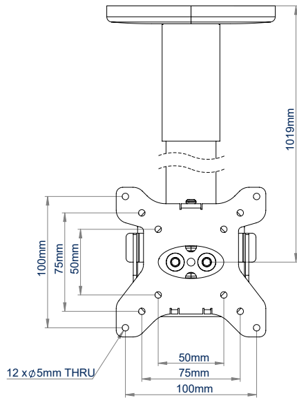
BT5970-FD100 FRONT VIEW
