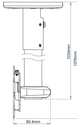
BT5970-FD100 SIDE VIEW
