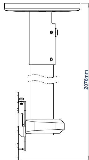
BT5970-FD200 SIDE VIEW
