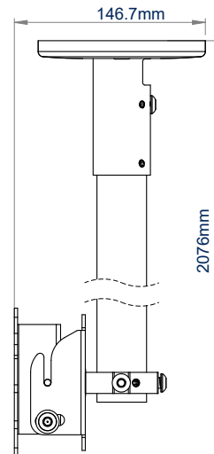
BT5971-FD200 SIDE VIEW
