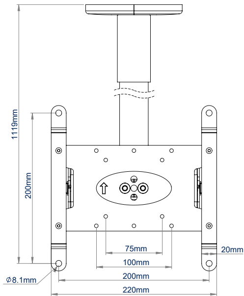
BT5972-FD100 FRONT VIEW (WITH INCLUDED VESA 200 ADAPTORS)
