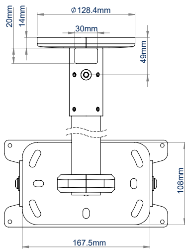
REAR VIEW (WITHOUT INCLUDED VESA 200 ADAPTORS)
