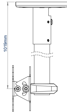
BT5972-FD100 SIDE VIEW (WITHOUT INCLUDED VESA 200 ADAPTORS)
