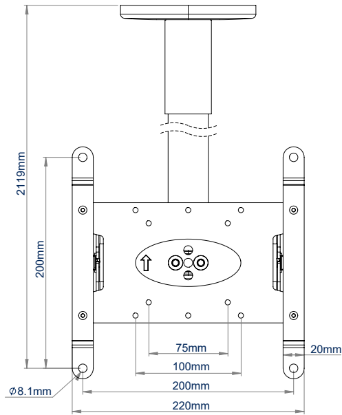
BT5972-FD200 FRONT VIEW (WITH INCLUDED VESA 200 ADAPTORS)
