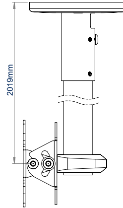
BT5972-FD200 SIDE VIEW (WITHOUT INCLUDED VESA 200 ADAPTORS)
