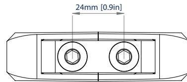
FRONT VIEW WITH COVER PLATE
