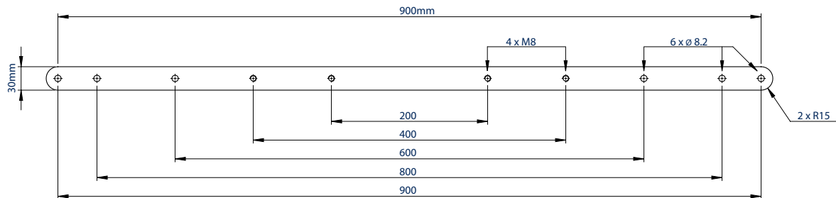
FRONT VIEW
