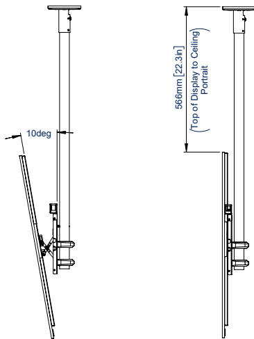
SIDE VIEW - TILT PORTRAIT ORIENTATION WITH SAMSUNG 32" E-PAPER
