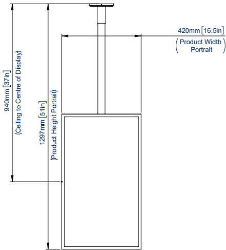
FRONT VIEW PORTRAIT ORIENTATION WITH SAMSUNG 32" E-PAPER
