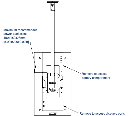
REAR VIEW WITH SAMSUNG 32" E-PAPER
