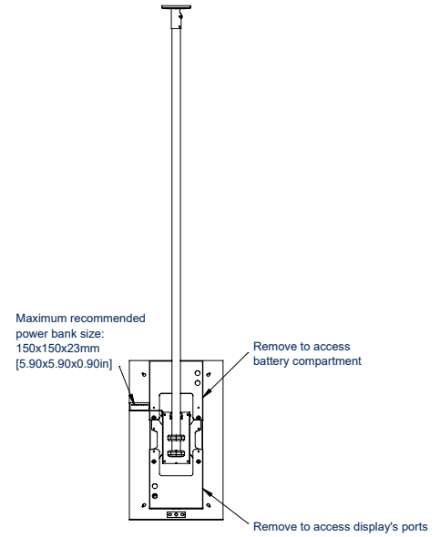
REAR VIEW WITH SAMSUNG 32" E-PAPER
