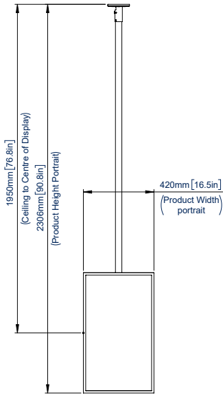
FRONT VIEW PORTRAIT ORIENTATION WITH SAMSUNG 32" E-PAPER
