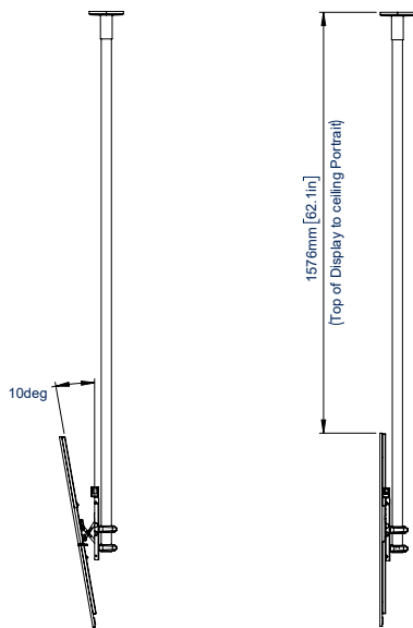
SIDE VIEW - TILT PORTRAIT ORIENTATION WITH SAMSUNG 32" E-PAPER
