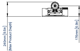
TOP VIEW PORTRAIT ORIENTATION WITH SAMSUNG 32" E-PAPER
