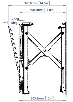
SIDE VIEW - OPEN STATE
