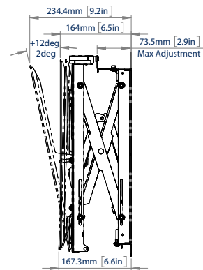
SIDE VIEW - CLOSED MAX ADJUSTMENT STATE
