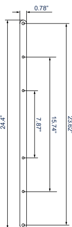
ADAPTOR ARMS
