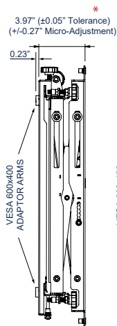
SIDE VIEW CLOSED
