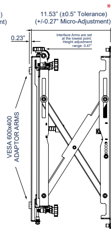
SIDE VIEW EXTENDED
