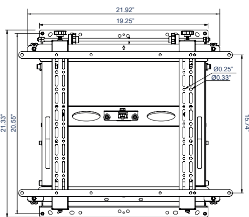
FRONT VIEW WITH ADAPTOR ARMS
