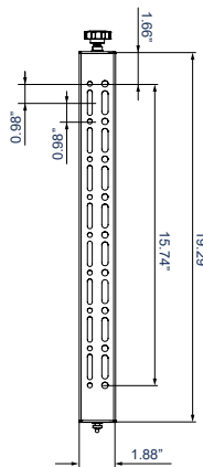
INTERFACE ARM
