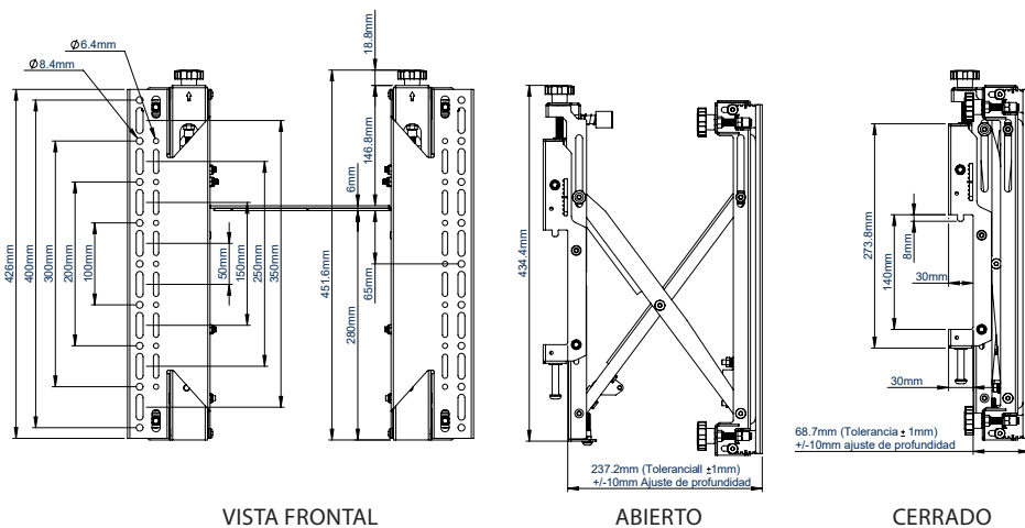
VISTA FRONTAL
