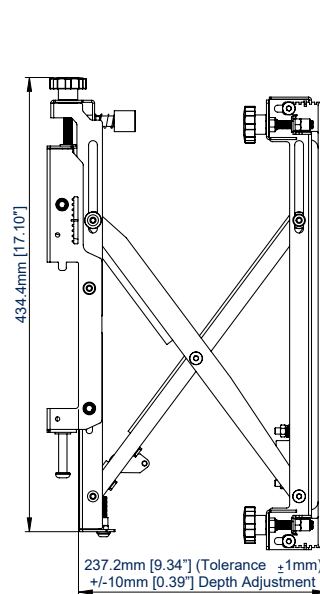
SIDE VIEW - EXTENDED
