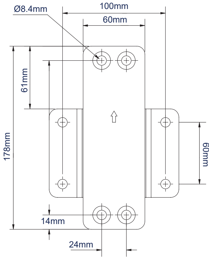
FRONT VIEW
