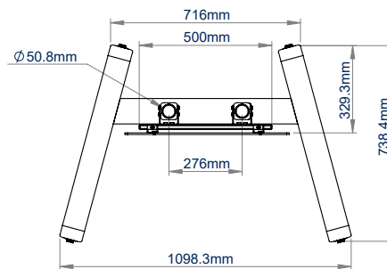
TROLLEY BASE
