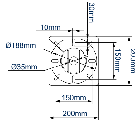
CEILING PLATE
