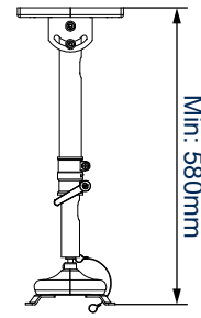
SIDE VIEW - MINIMUM EXTENSION
