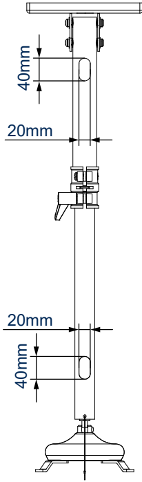
FRONT VIEW
