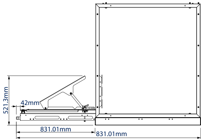
SIDE VIEW TRAY EXTENDED
