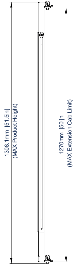
SIDE VIEW FULL EXTENSION
