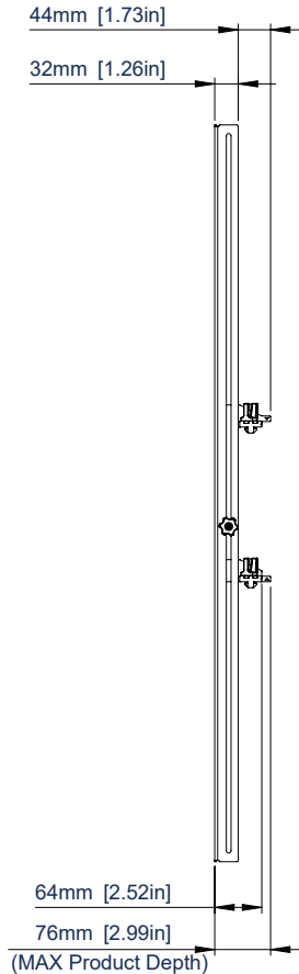
SIDE VIEW
