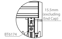
DETAIL D
