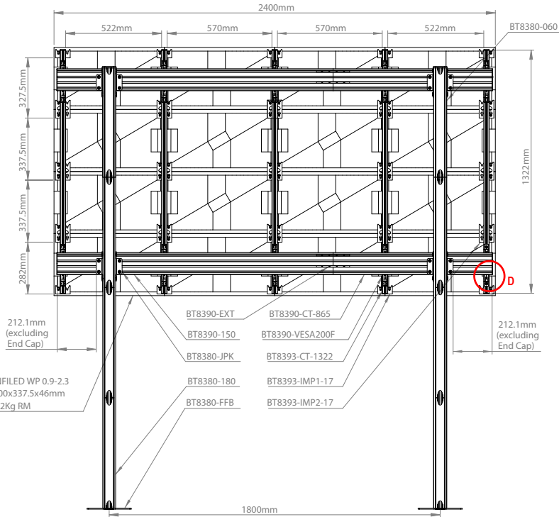
REAR VIEW
