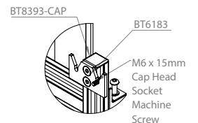
DETAIL E
