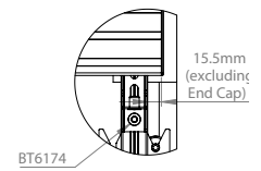
DETAIL D
