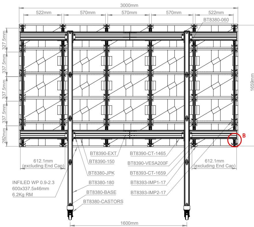
REAR VIEW
