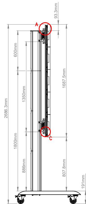
SIDE VIEW
