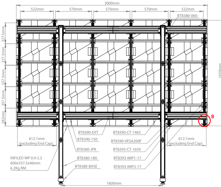
REAR VIEW
