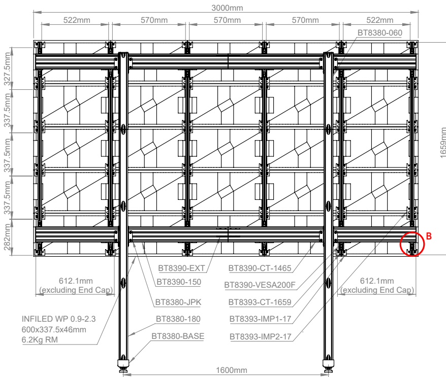
REAR VIEW
