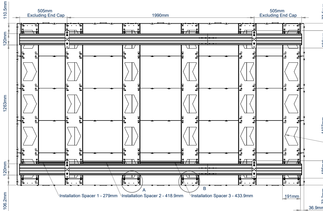
REAR VIEW
