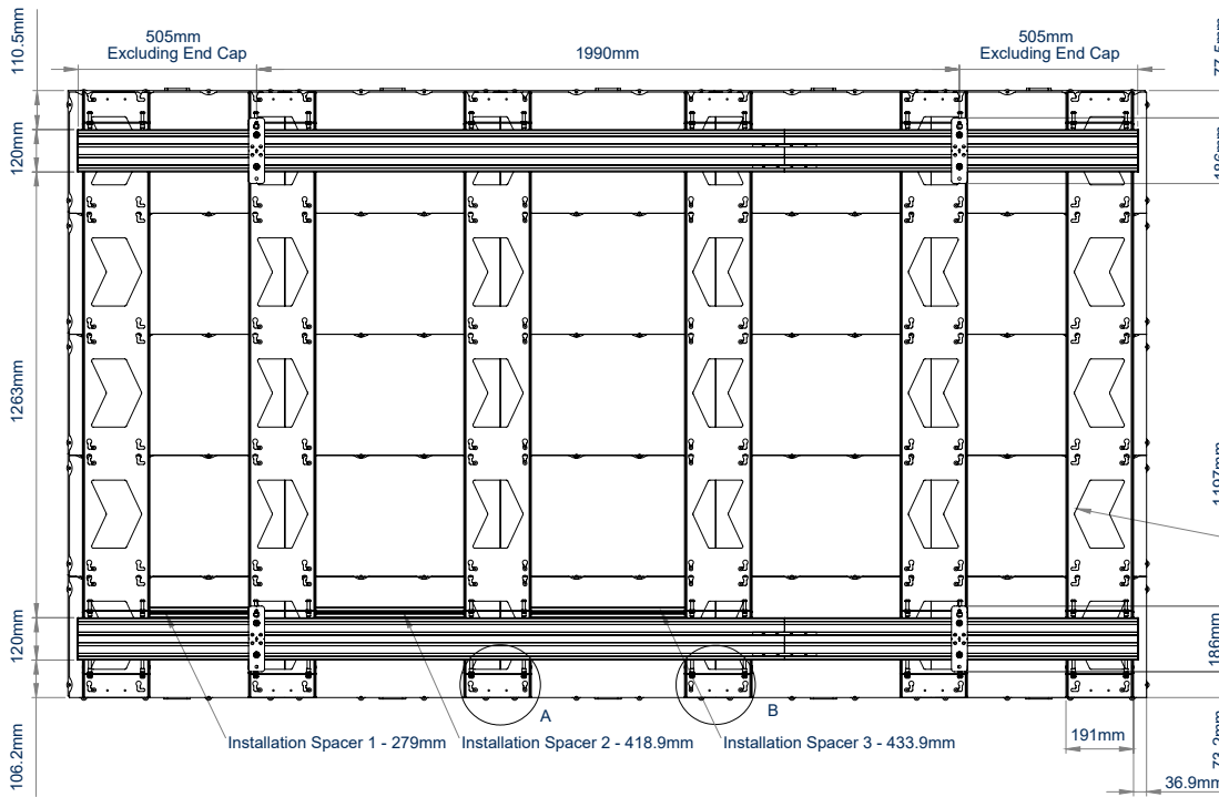
REAR VIEW
