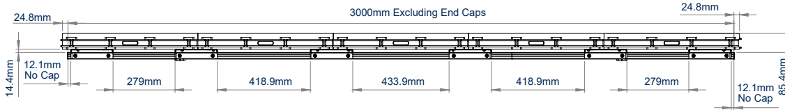
TOP VIEW
