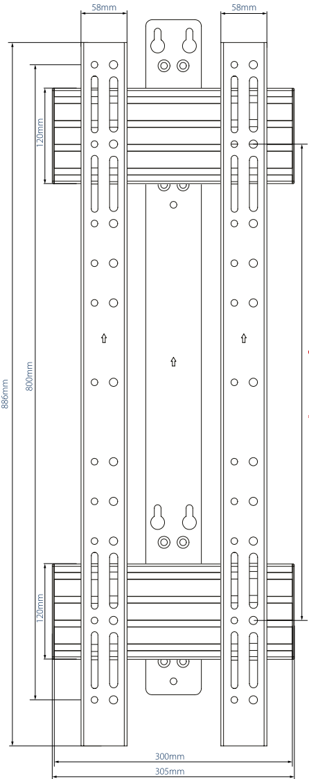
FRONT VIEW - HORIZONTAL RAILS & INTERFACE ARMS
