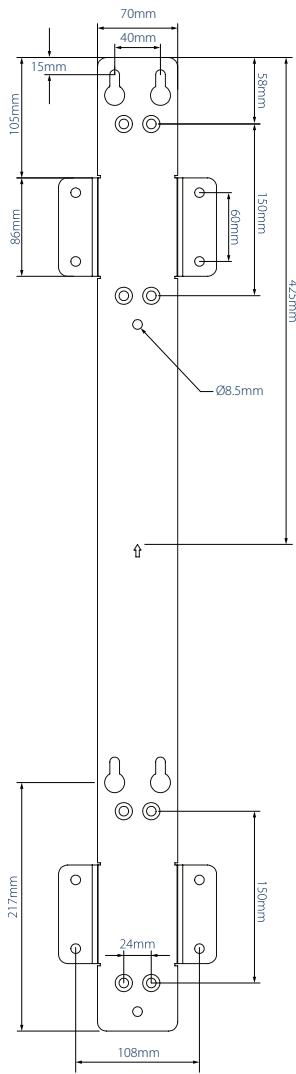
FRONT VIEW - WALL FIXING KIT
