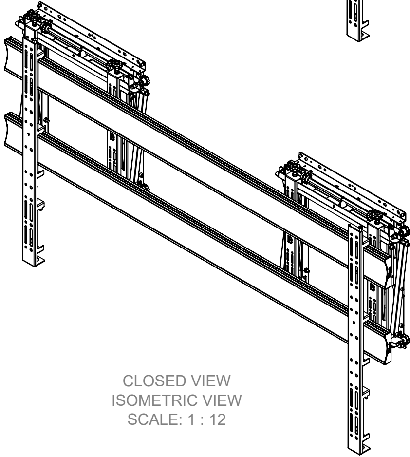
OPEN VIEW ISOMETRIC VIEW SCALE: 1 : 12
