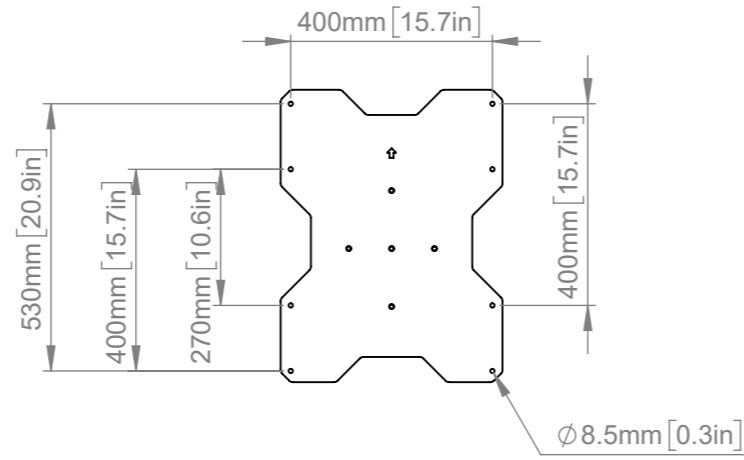
MOUNTING PLATE SCALE 1:15
