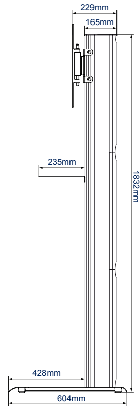
SIDE VIEW
