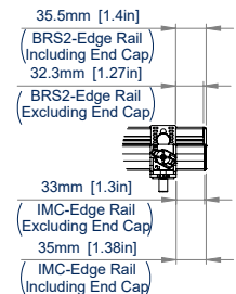
FRONT VIEW BT9240-BRS2
