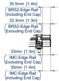
FRONT VIEW BT9240-BRS2
